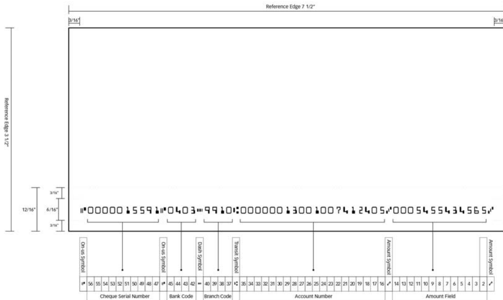
Figure 5: MICR line encoding locations and details (as in Annexure V)
