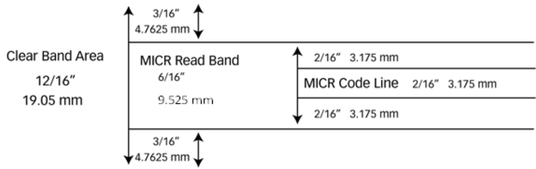
Figure 6: MICR line clear band location and dimensions
