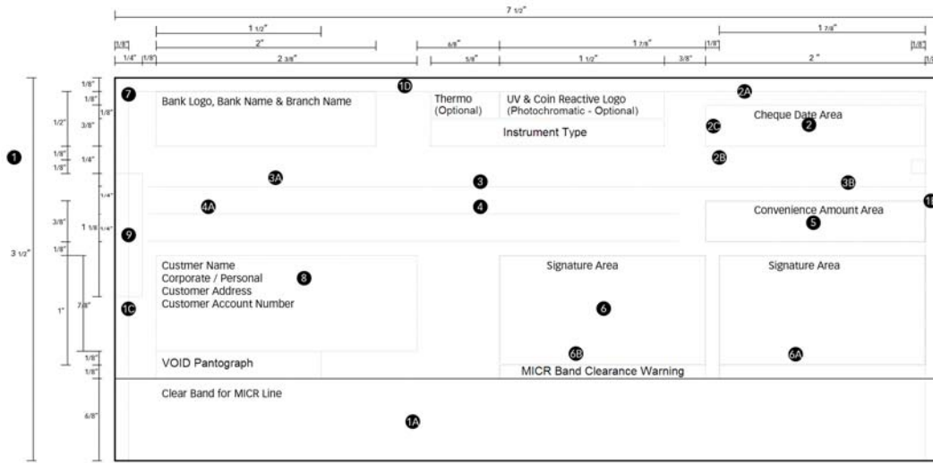
Figure 2: Cheque field locations (as in Annexure VIII)
