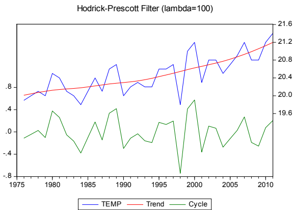
Figure 5: HP Filter for Temperature
