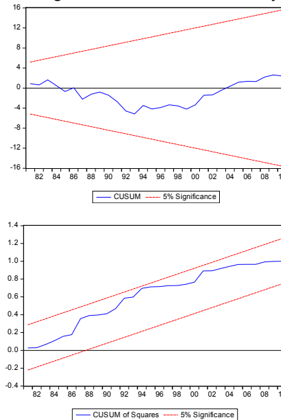
Figure 6: CUSUM test for stability
